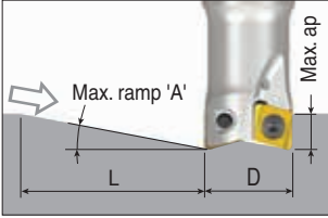
Straight ramping
