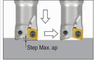
Step down
