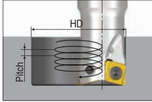
Helical ramping
